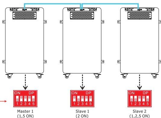
Example of three batteries in parallel
